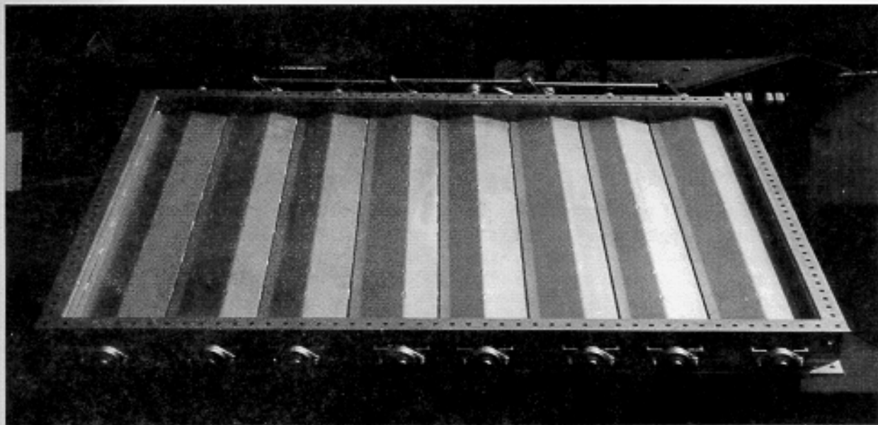
Fan control louver damper with opposed linkage, shown in the closed and partially open positions.
