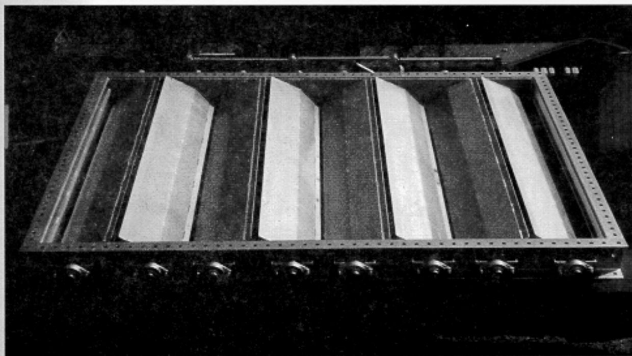
Fan control louver damper with opposed linkage, shown in the closed and partially open positions.
