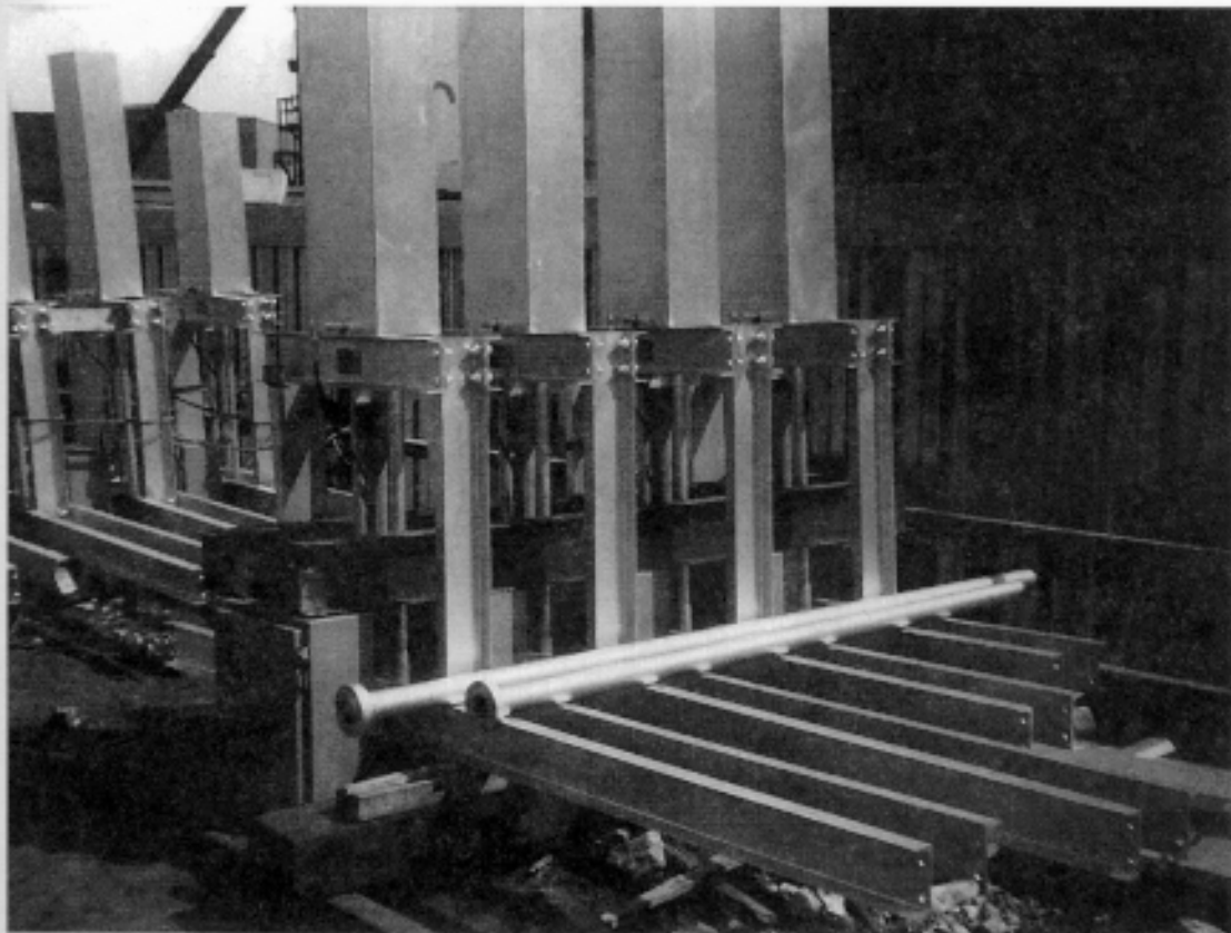
Baghouse poppets for a steel plant equipped with hydraulic cylinders and self contained pump units.
