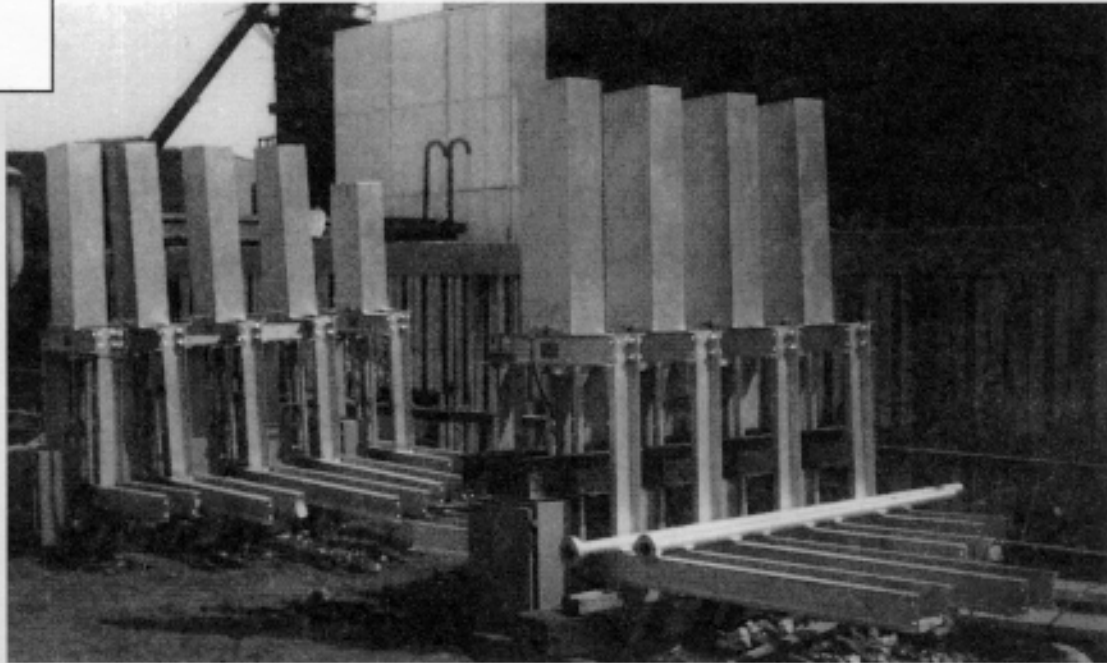
Baghouse poppets for a steel plant equipped with hydraulic cylinders and self contained pump units.
