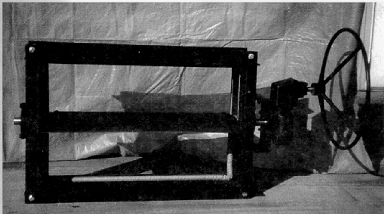
Single blade tadpole seat damper with gear drive and hand wheel.
