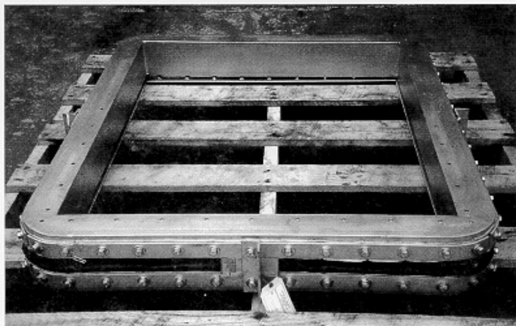
Radius corner, C frame expansion joint
