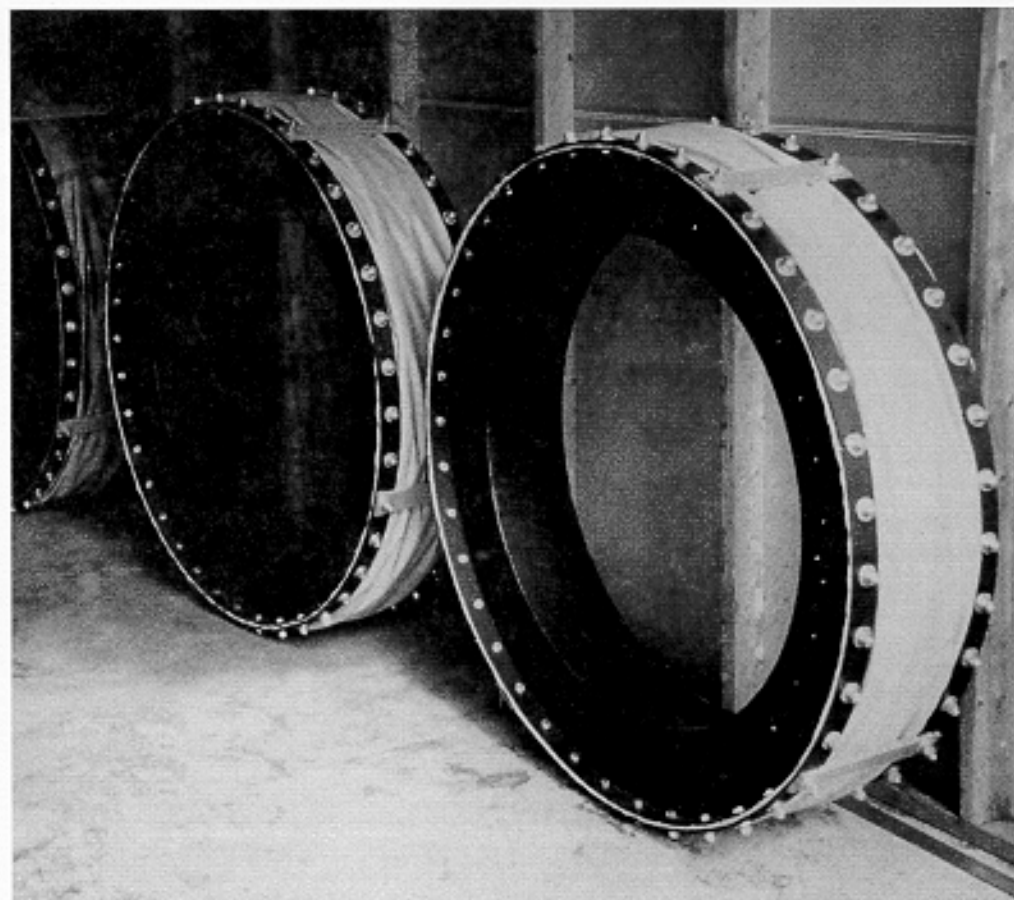
Round Z frame expansion joints
