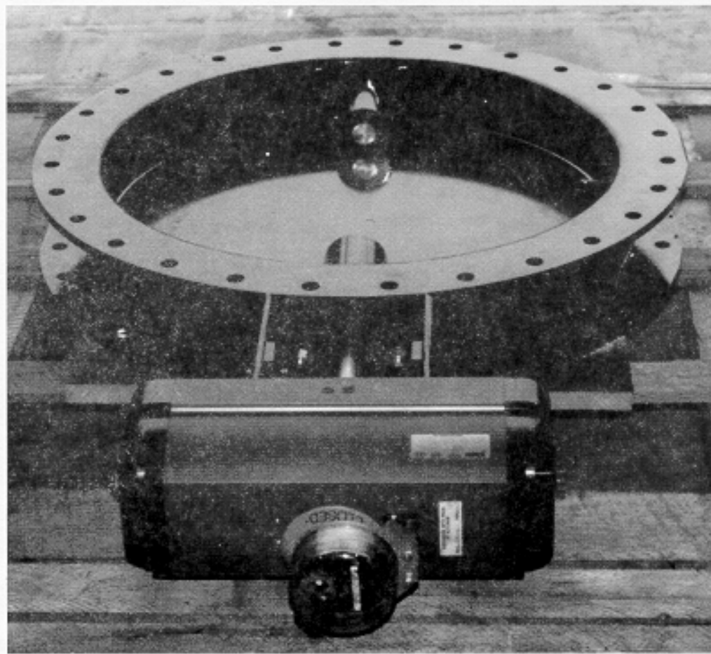
Teflon seated butterfly with pneumatic actuator.
